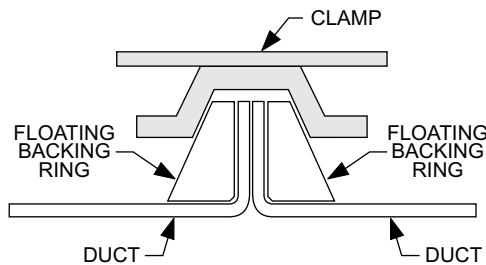
CROSS SECTION OF 4"-14" PSP-EZ™ JOINT
