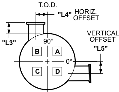
"D1" TAP OFFSET VIEW
