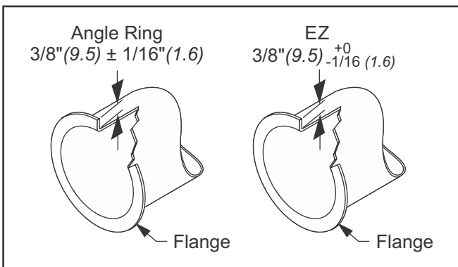
Fig. 20: Flange Height Dimensions & Tolerances
