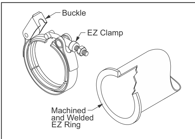
Fig. 16: 2" (50.8) & 3" (76.2) EZ configuration
