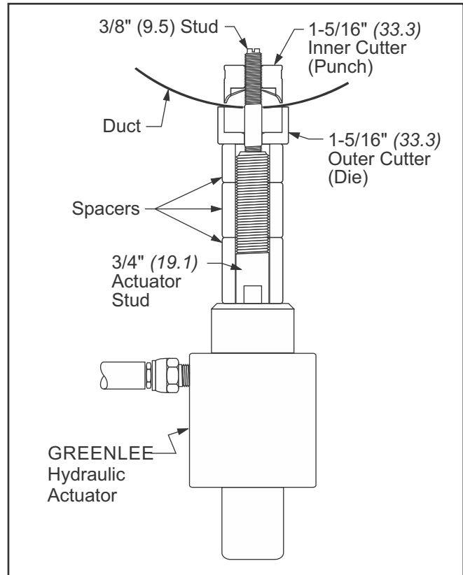
Fig. 35: 1-5/16" (33.3) Hydraulic Punch Configuration
