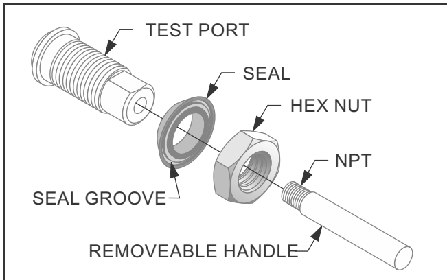
Fig. 42: 3/8" (9.5) Test Port Configuration
