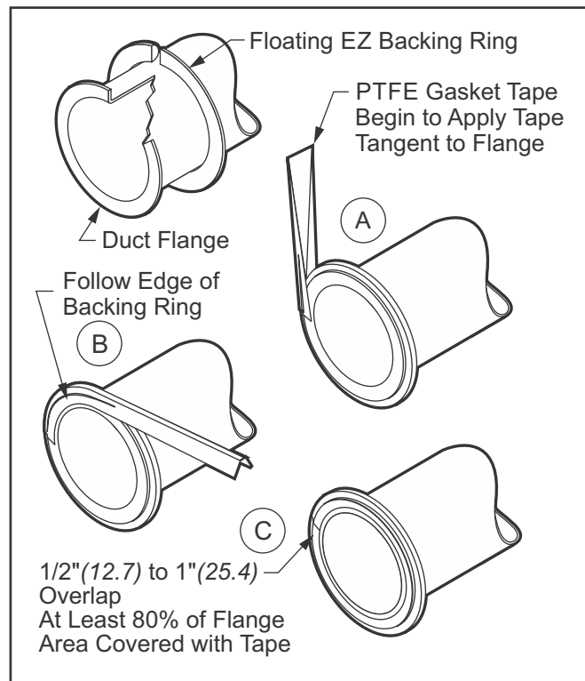
Fig. 13: Apply gasket for 4" (101.6) - 14" (355.6) EZ duct
