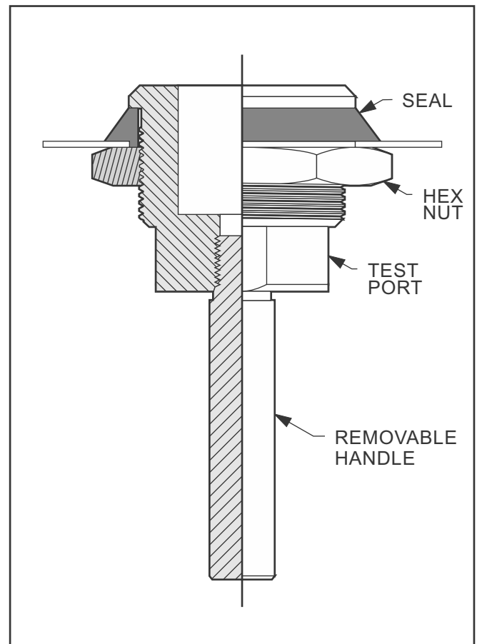
Fig. 48: 2" (50.8) Test Port Cut-away view
