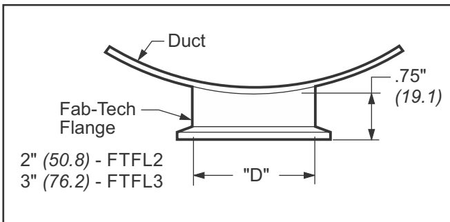
Fig. 49: Fab-Tech Flange Configuration
