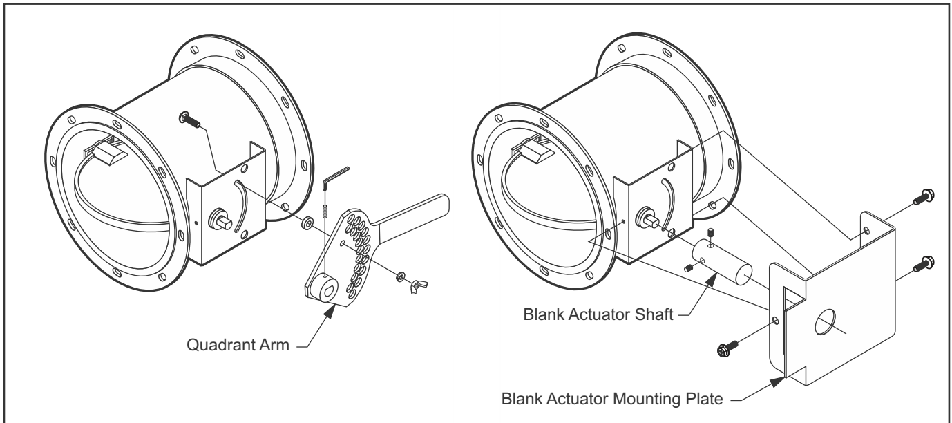
Fig. 51: 4" (101.6) - 14" (355.6) Industrial Damper Actuator Removal for Customer Supplied Actuator.
