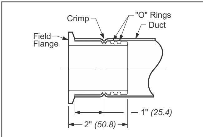
Fig. 22: EZ Field Flange Configuration
