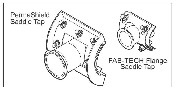
Fig. 27: PermaShield and EZ Saddle Taps
