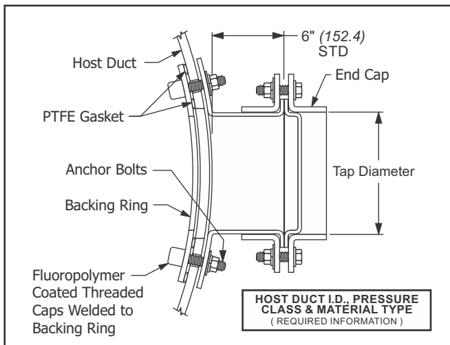
Fig. 28: Hot Tap - Section Through Duct
