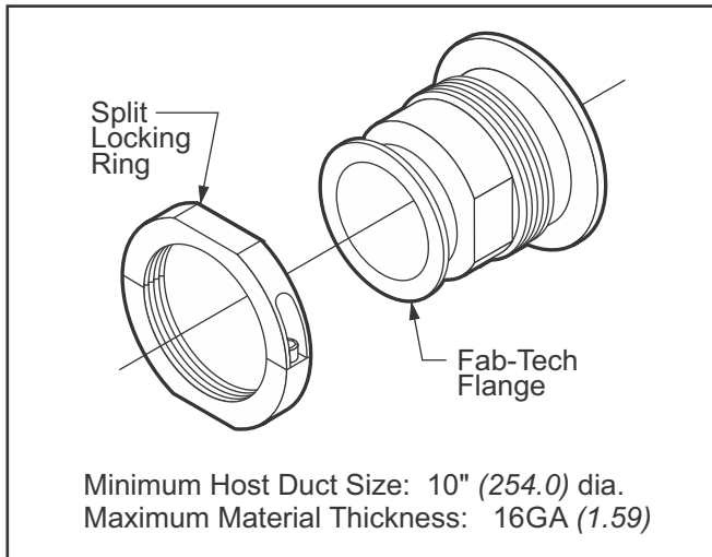
Fig. 30: Field Installed 2" (50.8) Fab-Tech Flange
