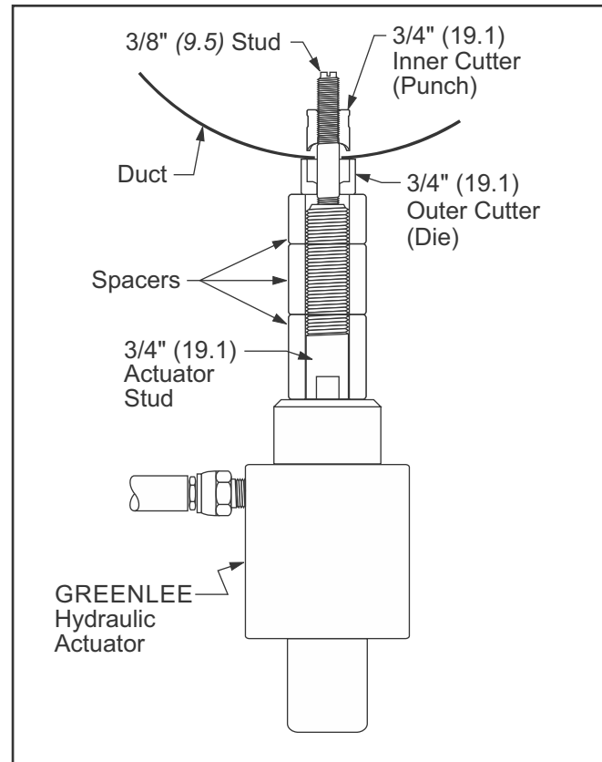
Fig. 31: 3/4" (19.1) Hydraulic Punch Configuration
