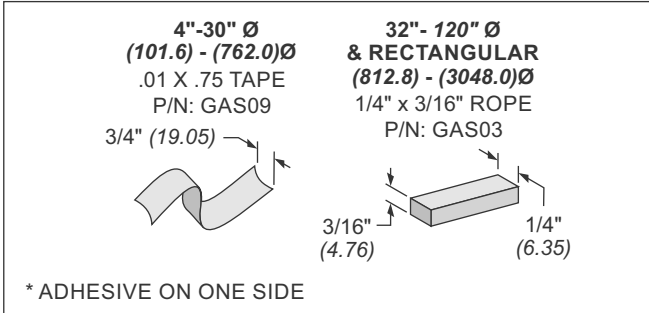
Fig. 6: Gasket size vs duct size
