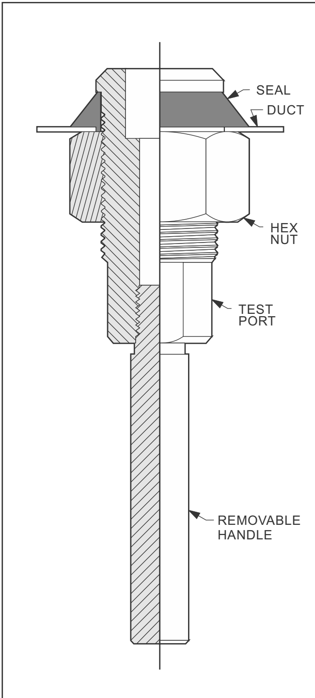
Fig. 47: 3/4" (19.1) Test Port Cut-away
