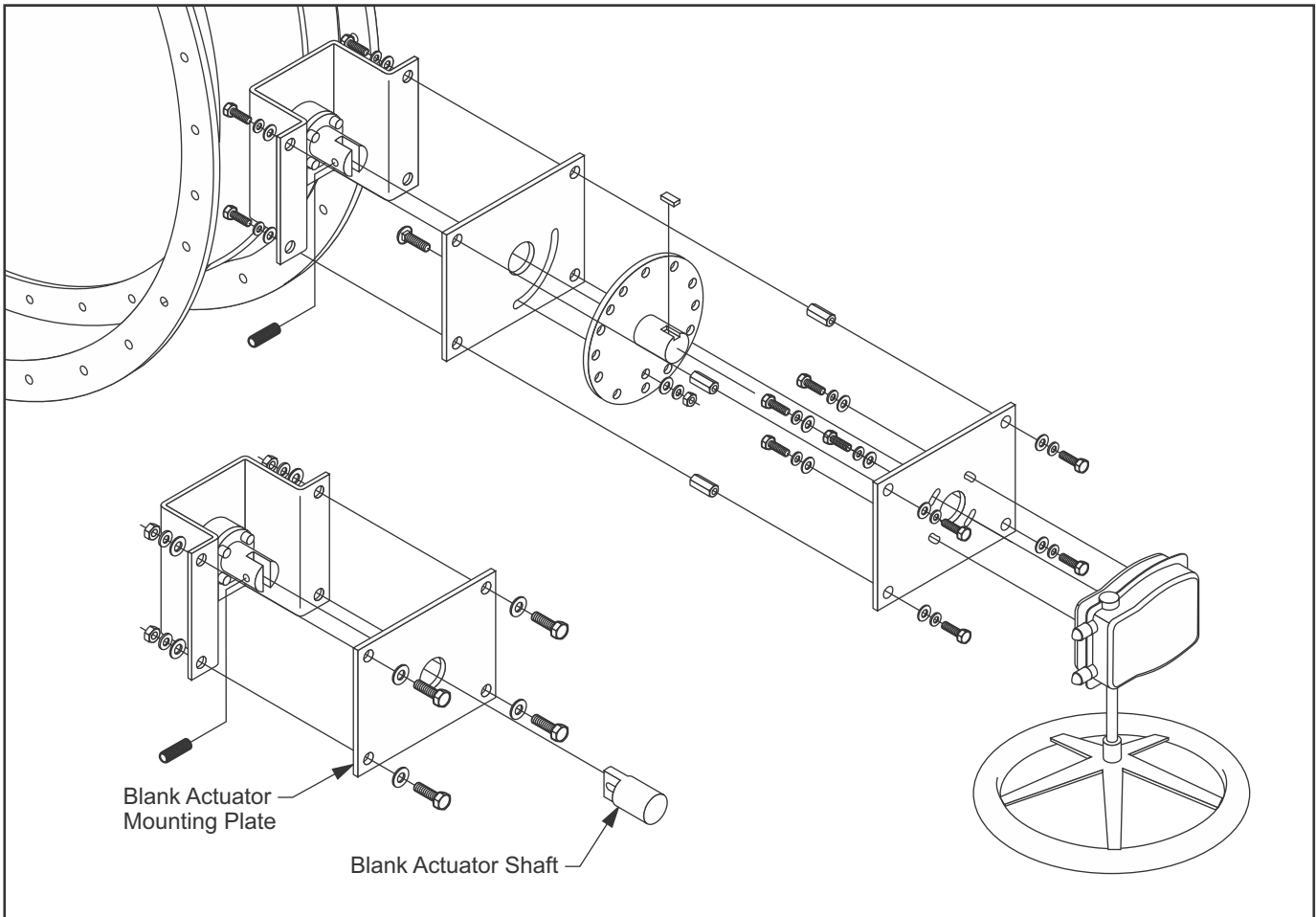
Fig. 53: 36" (914.4) - 48" (1219.2) Heavy Duty Industrial Damper Actuator Removal for Customer Supplied Actuator.
