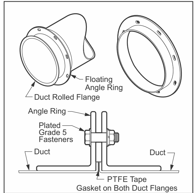
Fig. 4: Floating angle rings 16" (406.4) - 30" (762.0)
