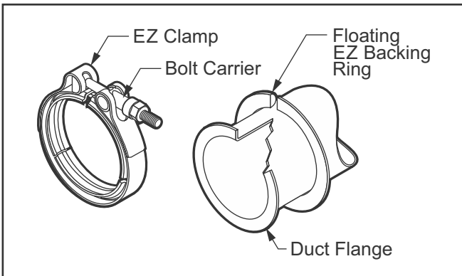
Fig. 12: 4" (101.6) - 14" (355.6) EZ configuration
