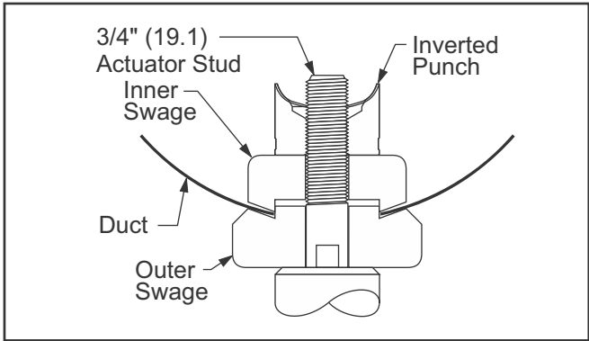
Fig. 33: 60mm Swage Configuration
