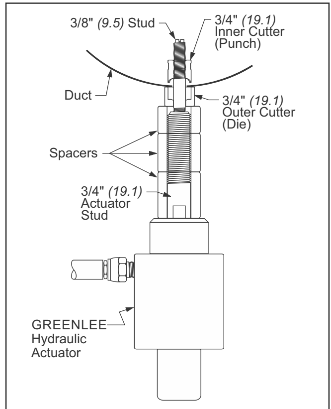
Fig. 38: 3/4" (19.1) Hydraulic Punch Configuration
