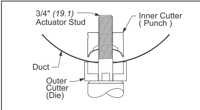
Fig. 39: 1-7/8" (47.6) Hydraulic Punch Configuration
