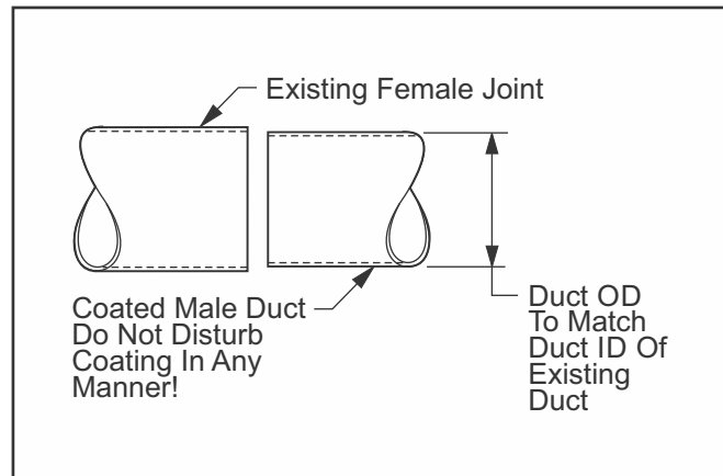
Fig. 2: Joining Dissimilar Unflanged Materials
