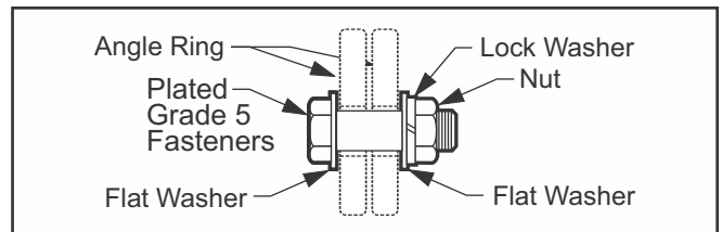
Fig. 11: Angle ring hardware configuration
