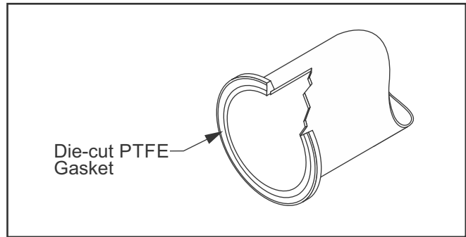
Fig. 17: Apply gasket for 2" (50.8) & 3" (76.2) EZ duct
