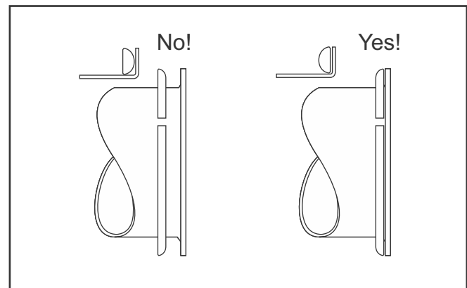
Fig. 21: EZ Backing Ring Position
