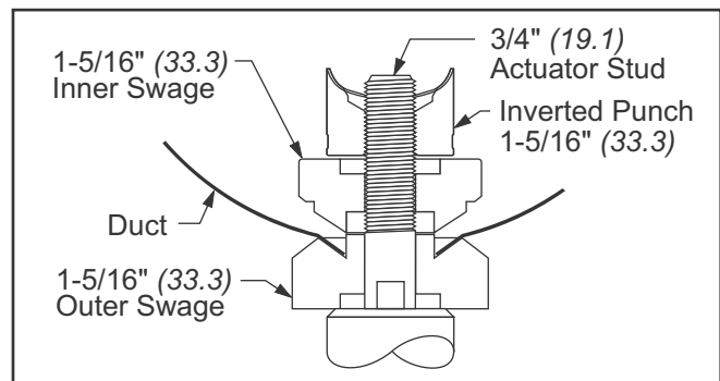
Fig. 36: 1-5/16" (33.3) Swage Configuration
