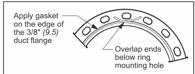
Fig. 10: Gasket installation for floating & fixed rings
