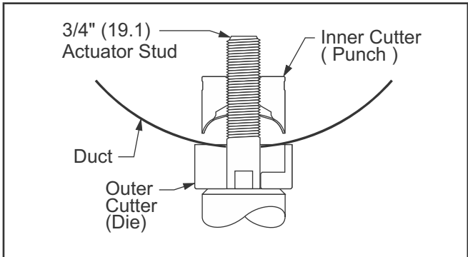
Fig. 32: 60mm Hydraulic Punch Configuration
