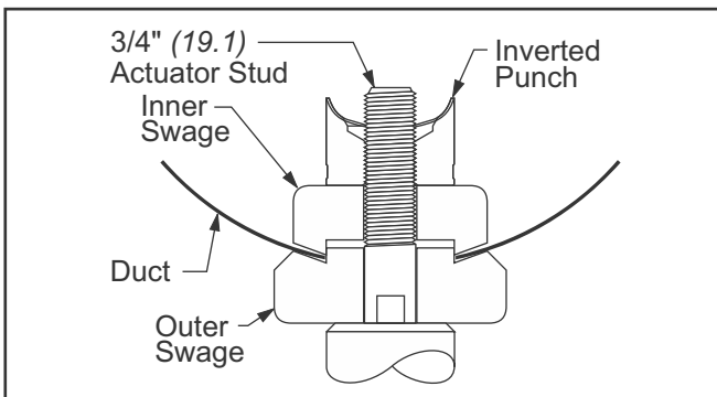
Fig. 40: 1-7/8" (47.6) Swage Configuration
