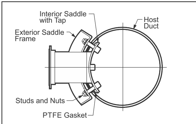
Fig. 25: Saddle Tap Configuration
