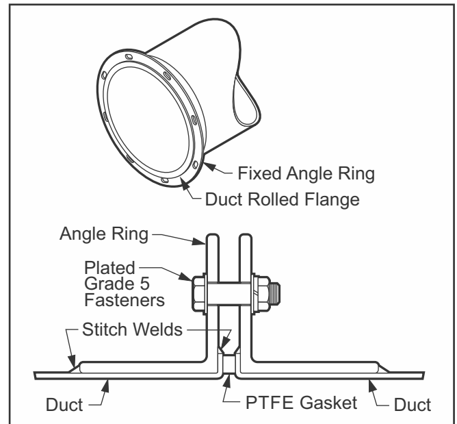
Fig. 5: Fixed angle rings 32" (812.8) - 120" (3048.0)
