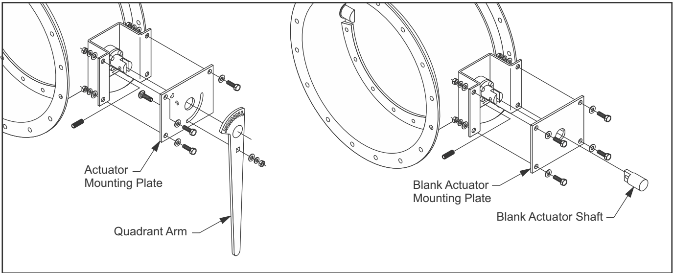
Fig. 52: 16" (406.4) - 34" (863.6) Heavy Duty Industrial Damper Actuator Removal for Customer Supplied Actuator.
