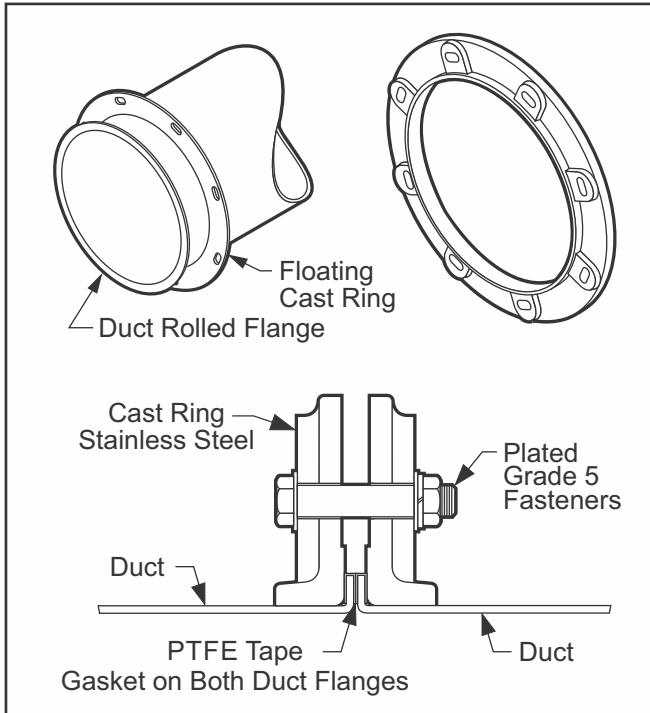
Fig. 3: Floating cast rings 4" (101.6) - 14" (355.6)
