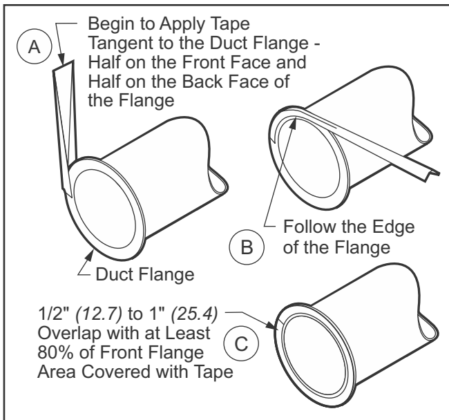
Fig. 9: Apply gasket for 4" (101.6) to 30" (762.0) duct
